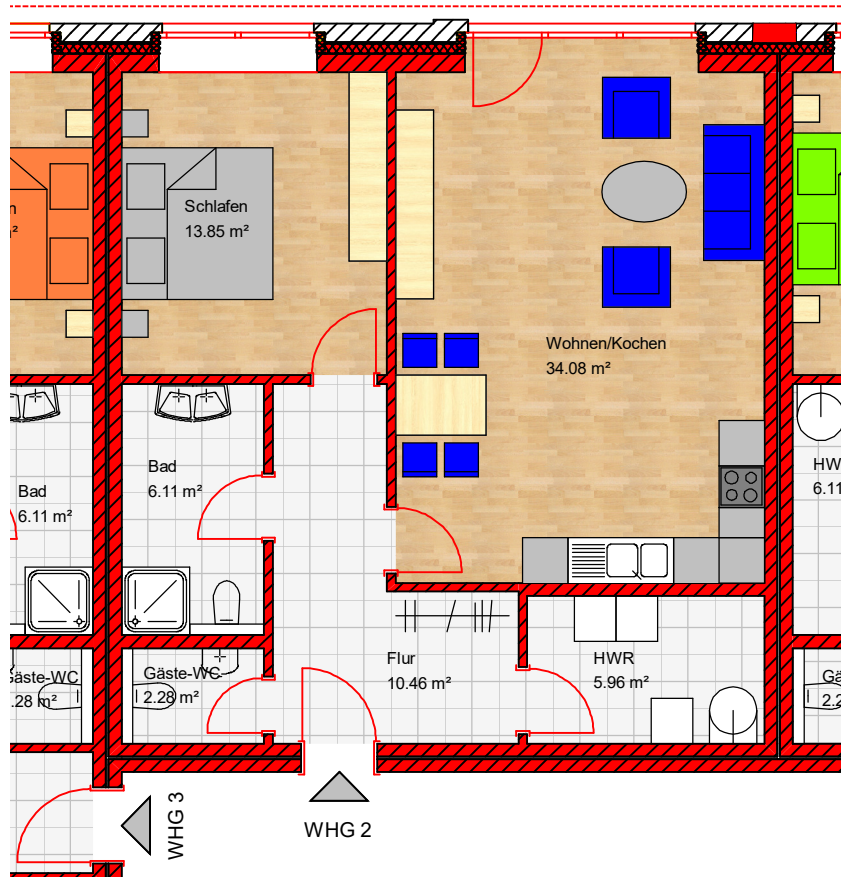
Grundriss WHG 2, 1:100
