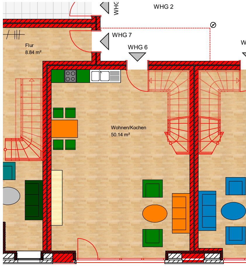
Grundriss WHG 6, 1:100
